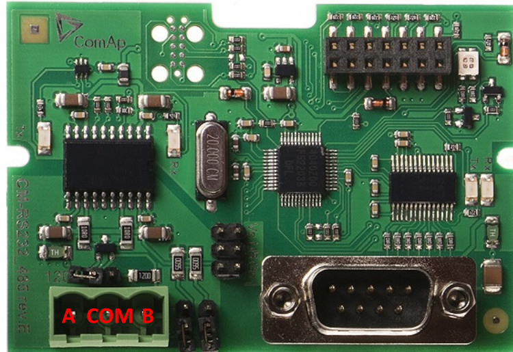
Image 1.1 CM-RS232-485 interface
